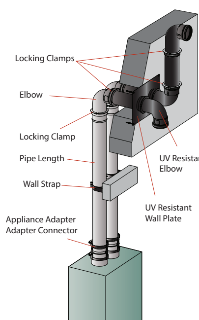
Horizontal Twin Pipe Elbow Termination
