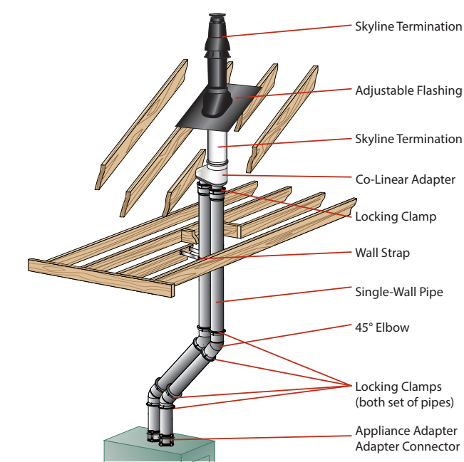
Twin Pipe with Concentric Termination
