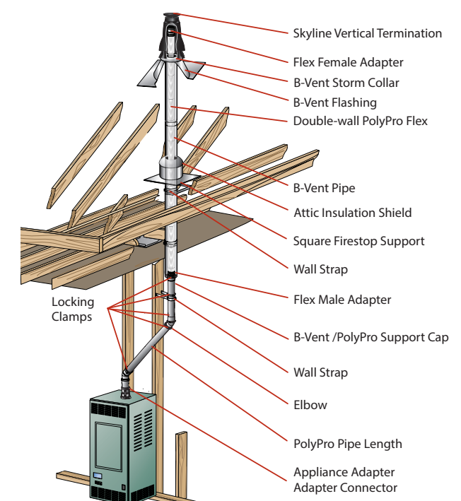
Flex Through B Vent as a Chase
