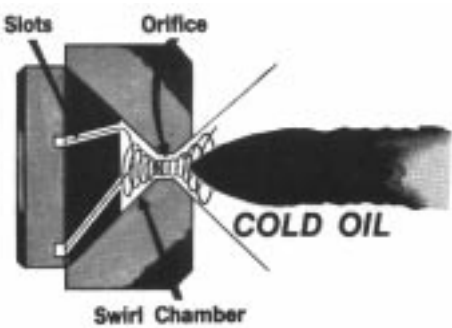
Figure 15 Cold Oil
