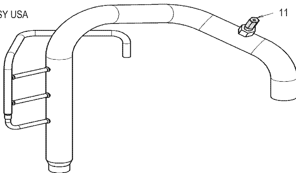
REFRIGERANT PIPE ASSY INJECTION
