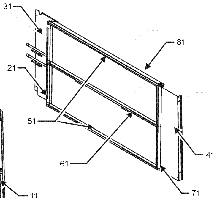
EVAPORATOR ASSEMBLY
