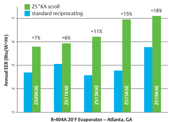
Annual Energy Efficiency Comparison ZS*KA scroll vs. standard reciprocating
