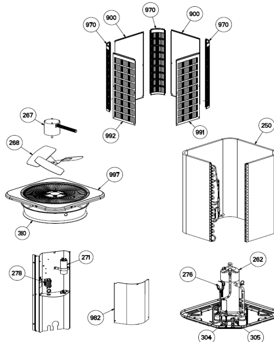
"RSG14SERIES" SINGLE PHASE AND 3 PHASE AIR CONDITIONER PARTS LIST
