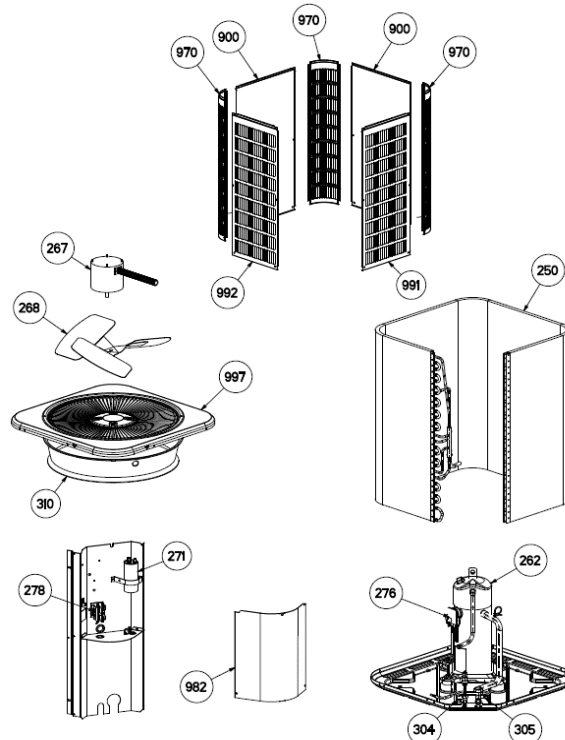
"RSG14SERIES" SINGLE PHASE AND 3 PHASE AIR CONDITIONER PARTS LIST
