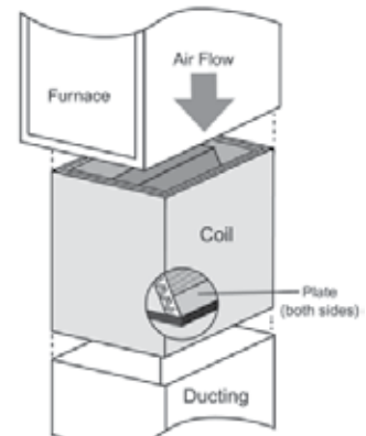
Fig 5A-2. Downflow Application
