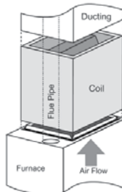
Fig 5A-1. Upflow Application
