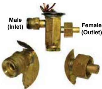
III-5. Remove the valve from the box and note the location of the inlet side (threaded male port) and the outlet side (female swivel nut port).
