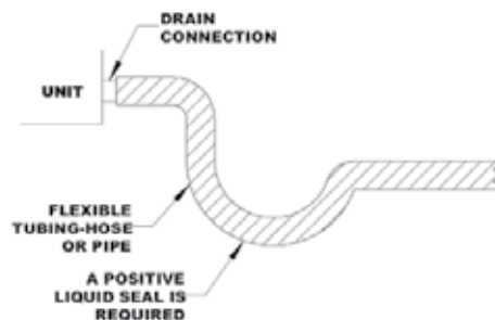
Fig 4-1. Typical drain line trap set up
