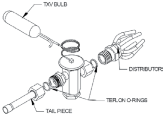
Fig 7B-1. Components of a typical TXV assembly
