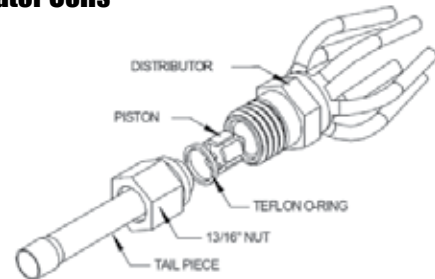
Fig 7A-1. Flowrator assembly components
