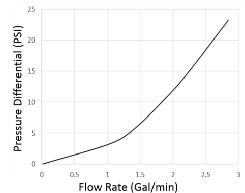
Flow Curve
