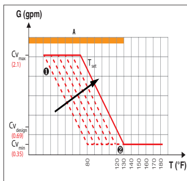
Thermostatic control with check valve, 11614xAC series
