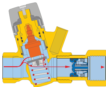
Thermostatic control with check valve, 11614xAC series
