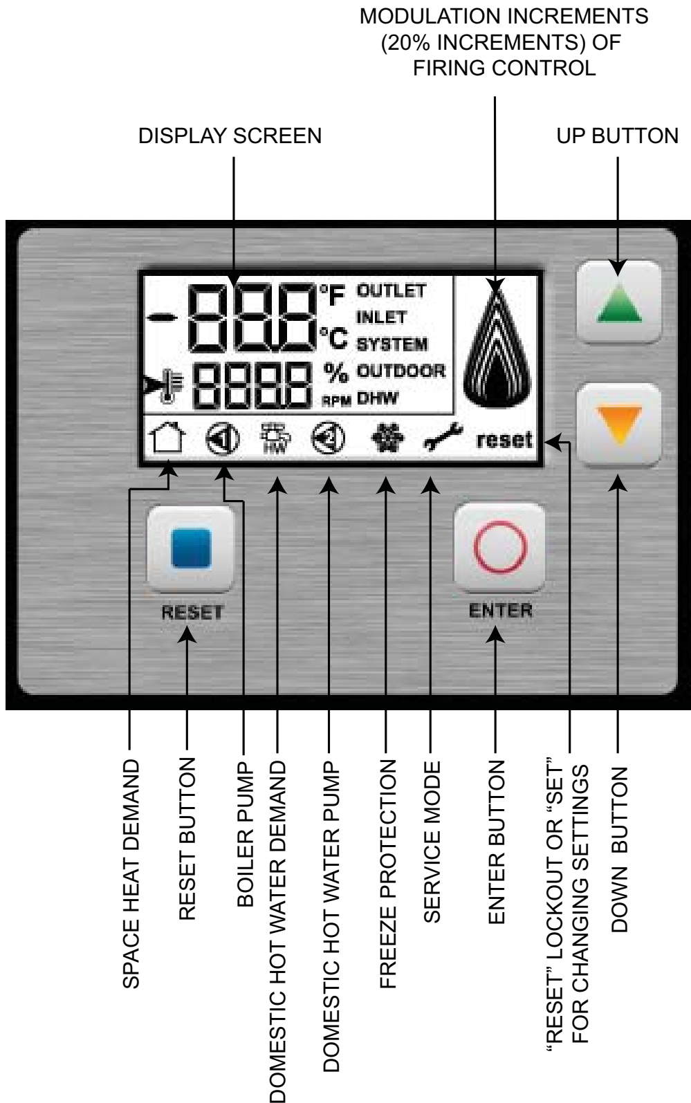
Figure 4-1 Control Panel Indicators
