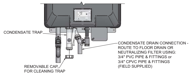
Figure 2-2 Condensate Disposal
