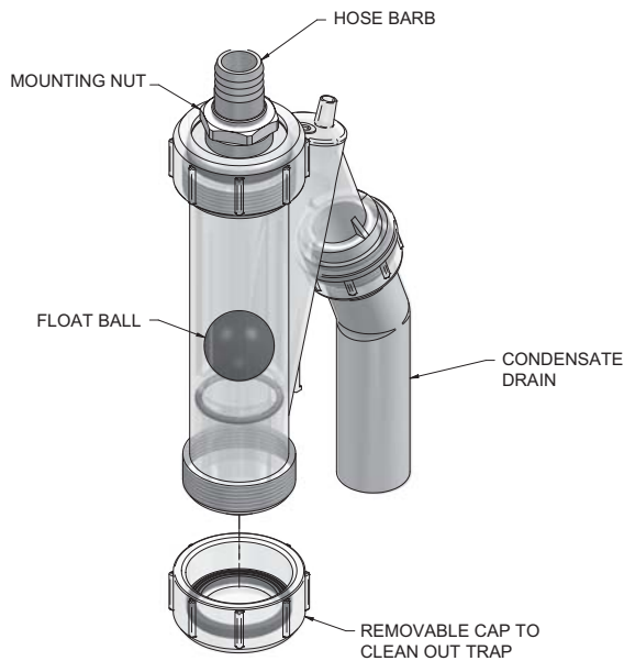
Figure 2-1 Condensate Trap
