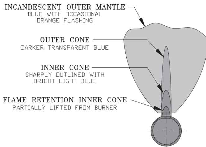
Figure 9: 1 Inch Main Burner Flame
