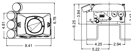
VP200 Pneumatic Positioner
