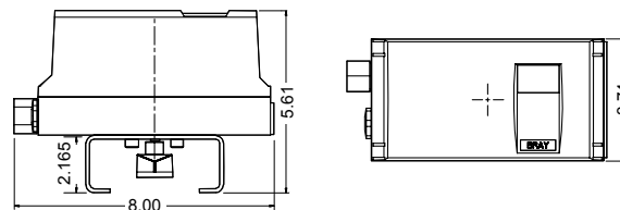
Series 6A Electro Pneumatic Positioner
