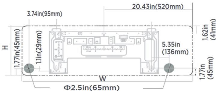
Indoor unit dimensions(WxH): 38.2in(971mm)x12.6in(321mm)
