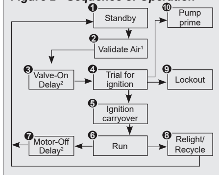
Figure 2 - Sequence of Operation
