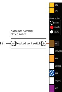
Figure 13 - 120Vac Blocked Vent Wiring
