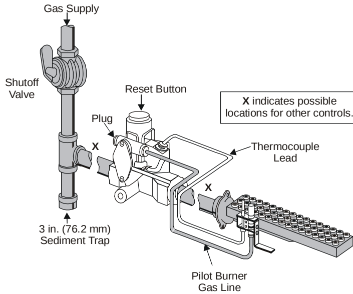
Figure 1: Typical Installation of an H15 Valve with Internal Pilot Gas Flow (Models H15_A and H15_B)
