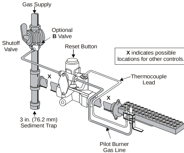
Figure 3: Typical Installation of an H15 Valve with External Pilot Gas Flow (Models H15_Q and H15_R)
