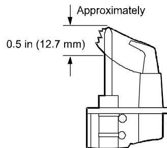
Figure 4: Flame Position
