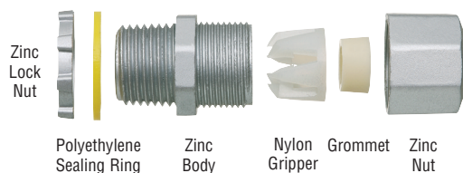
LPCG50Z Exploded View
