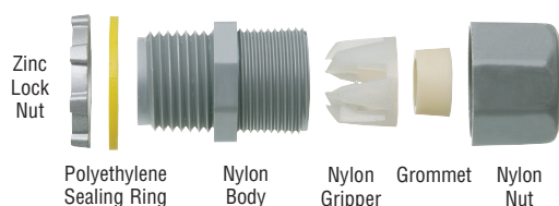
LPCG50 Exploded View
