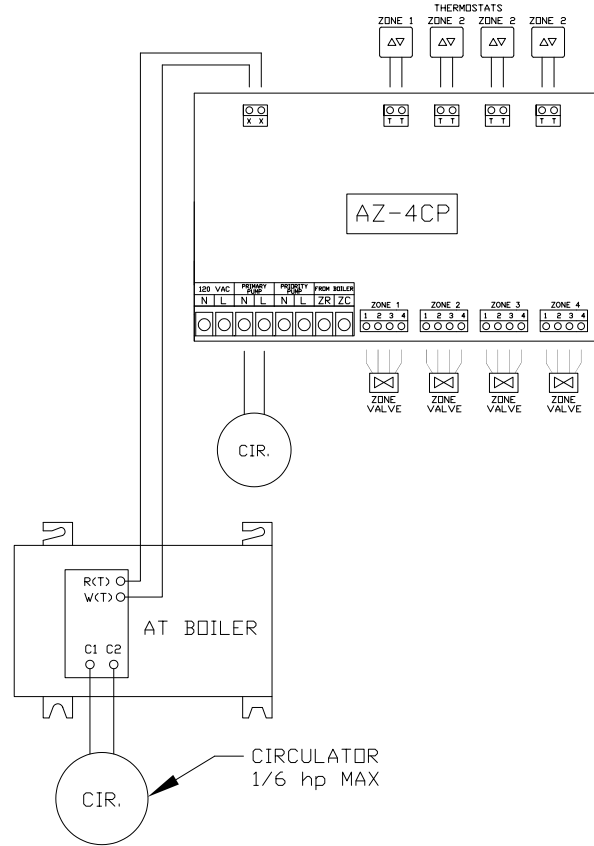
Figure 15 - Three Zones with Circulators
