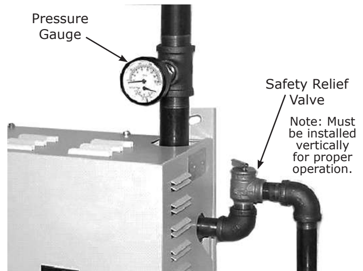
Figure 1A - Safety Relief Valve
