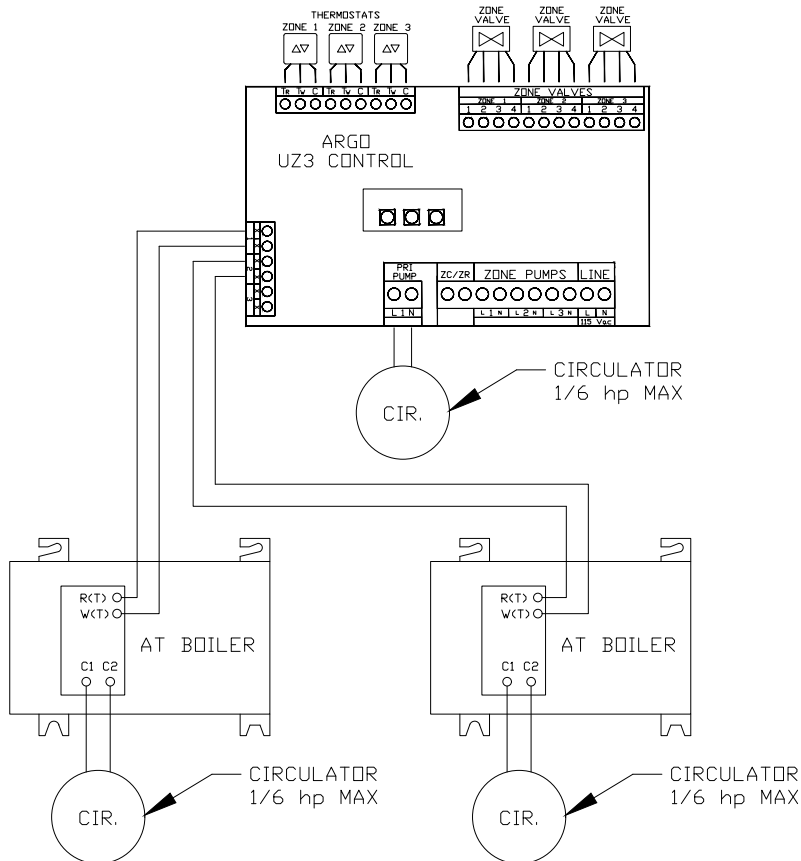
Figure 13 - Three Zones with Zone Control Valves - 2 Boilers
