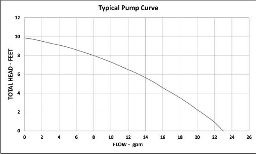
Figure 1B - Typical Pump Curve
