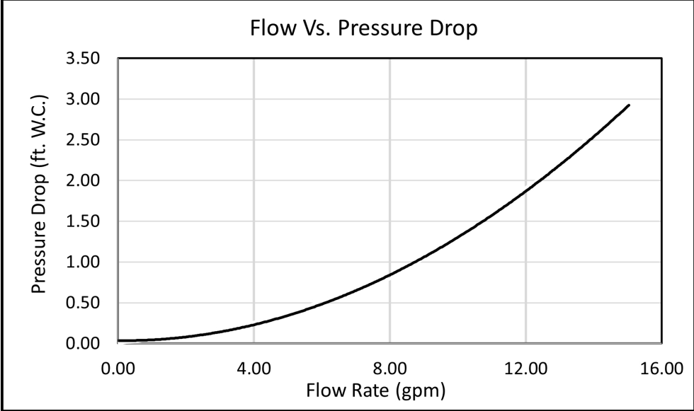
Figure 1C - Boiler Pressure Drop
