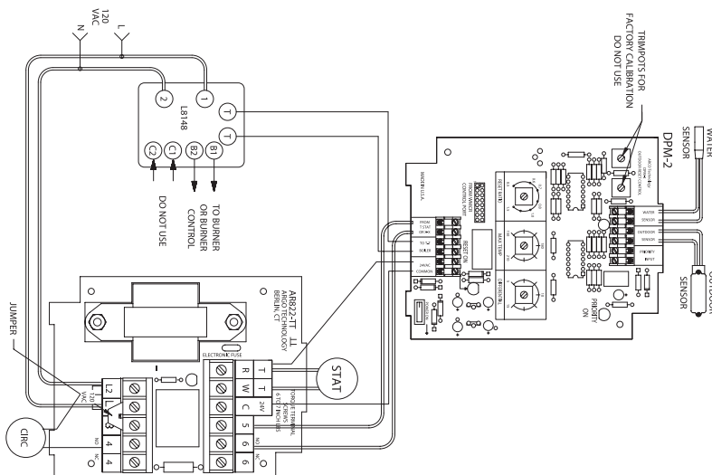
Typical Wiring Application Using DPM-2 Outside Reset With ARGO AR822-II Relay Control
