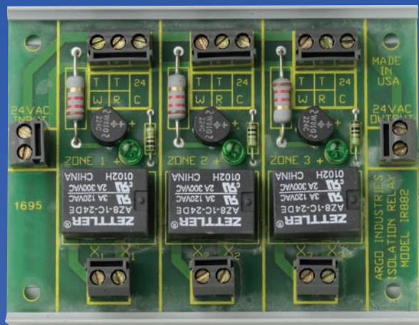
IR882 3-Zone
