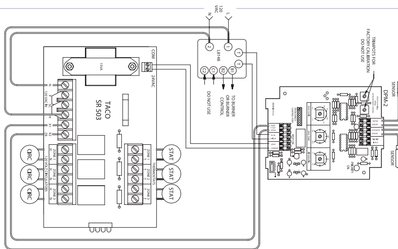
Typical Wiring Application Using DPM-2 Outside Reset With TACO SR 503 Relay Control
