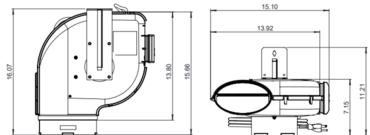
Figure 1 - Overall Dimensions (inches) Model V42SNX
