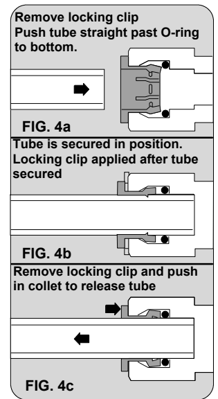
FIG. 4 Quick Connect / Push-in Connector
