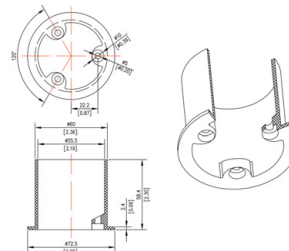
3" SEAL - Part 2
