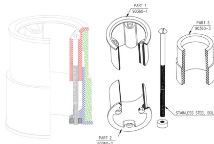
4" SEAL
