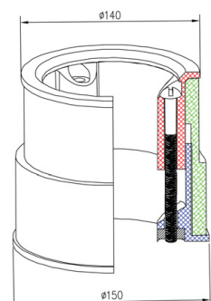
6" SEAL
