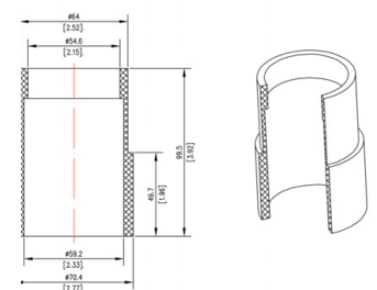
3" SEAL - Part 3
