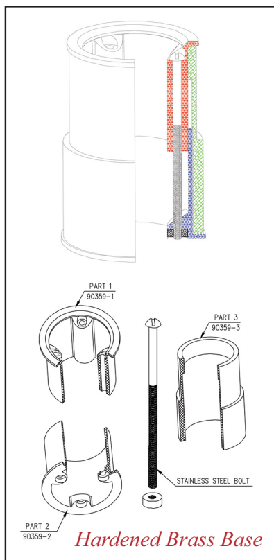
3" SEAL - Part 1
