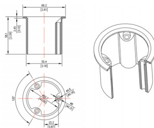
3" SEAL - Part 1
