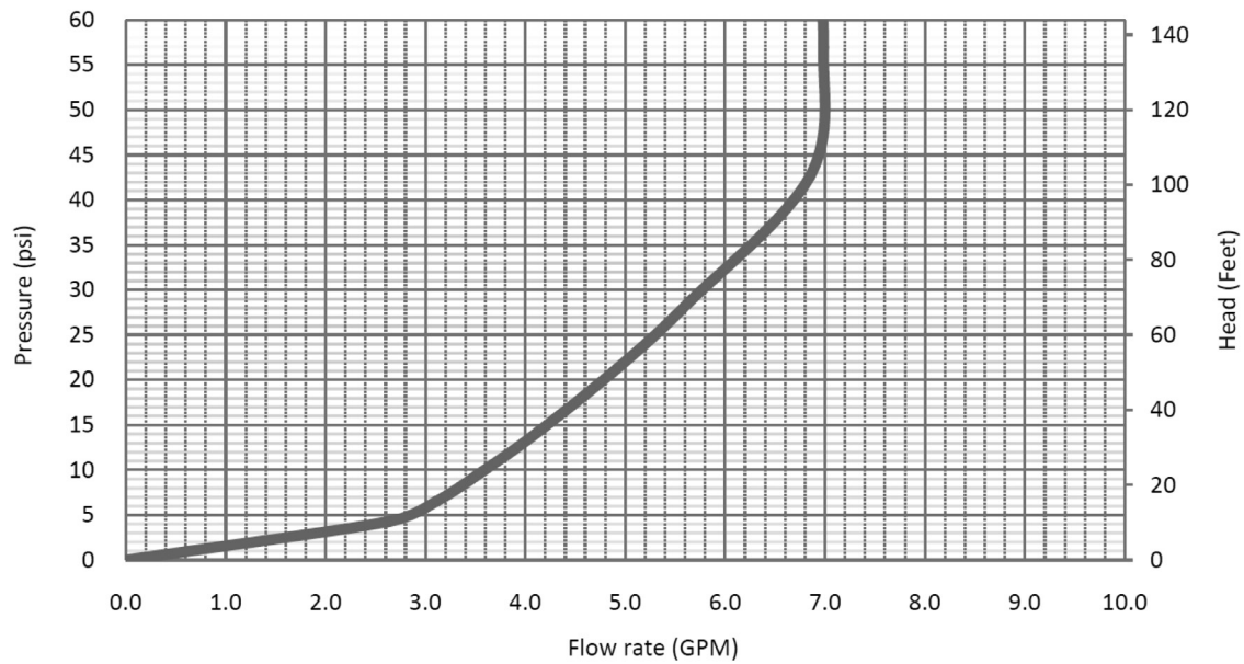
Pressure loss
