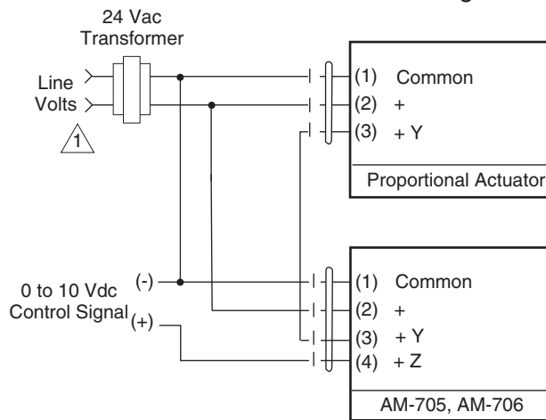
Figure-13 AM-705 and AM-706 Wiring Diagram.
