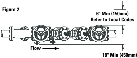
HORIZONTAL INSTALLATION OF THE DC SERIES 850, LF850 & DCDA SERIES 856, 856ST (Top View, Shown With Strainer)
