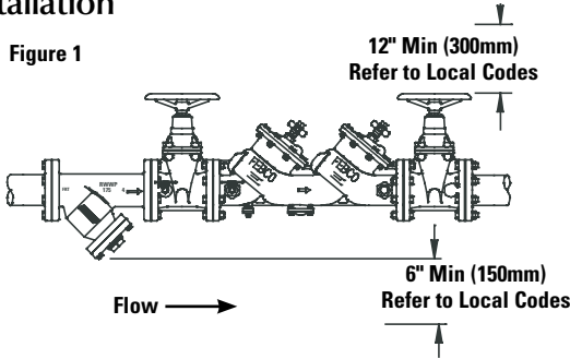
HORIZONTAL INSTALLATION OF THE DC SERIES 850, LF850 & DCDA SERIES 856, 856ST (Front View, Shown With Strainer)
