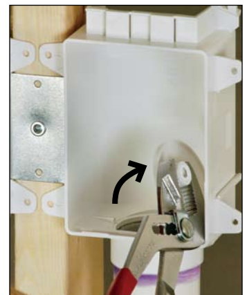
Drain Knockout
