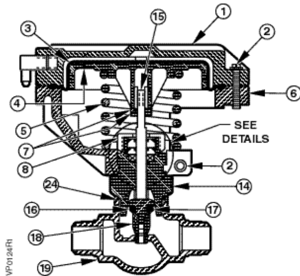
Figure 3. Normally Open.
