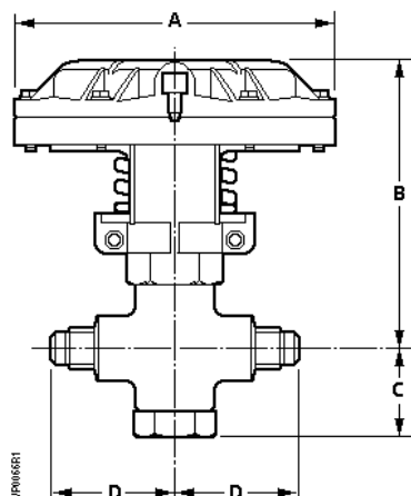
Figure 7. Normally Closed.
