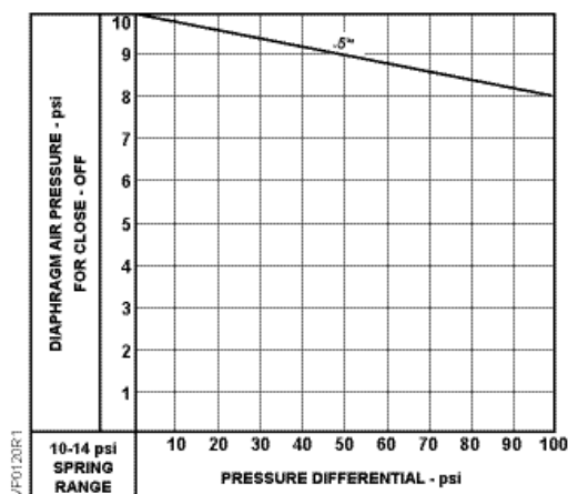
Normally Closed
