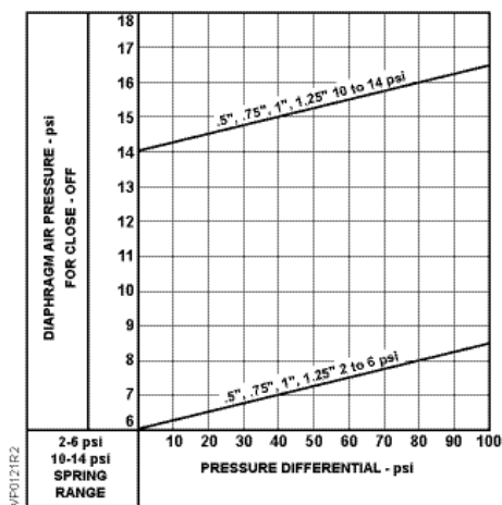
Normally Open
