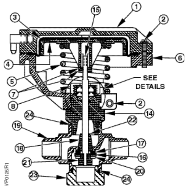
Figure 5. Normally Closed.
