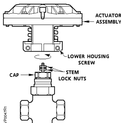
Figure 2. Actuator Replacement.
