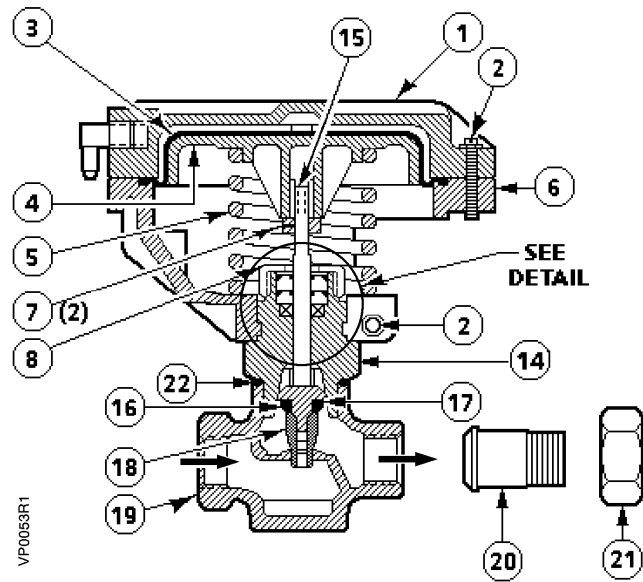
Figure 4. Angle Union Outlet, Normally Open.
