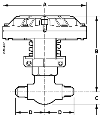
Figure 6. Normally Open.
