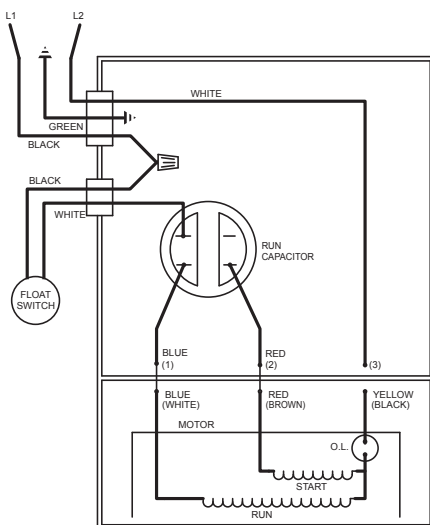
WIRING DIAGRAM FOR MODELS WD405 ALL REVISIONS
