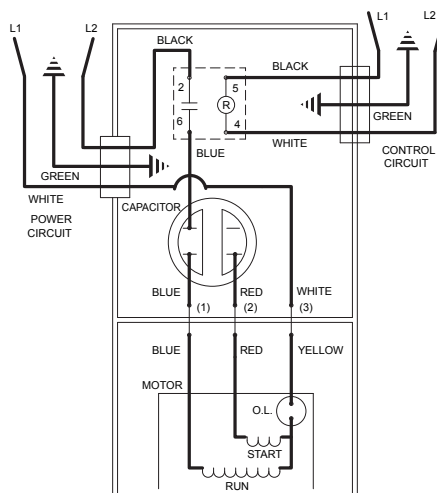
WIRING DIAGRAM FOR MODELS XE405 ALL REVISIONS
