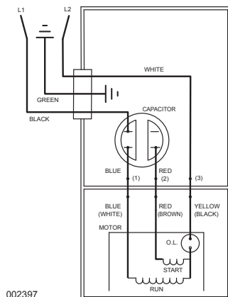
WIRING DIAGRAM FOR MODELS E405 ALL REVISIONS
