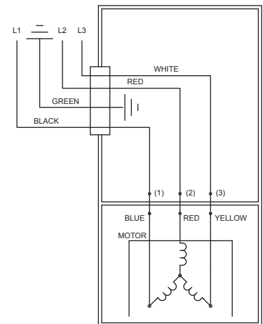
WIRING DIAGRAM FOR MODELS I405, J405, F405, G405 AND BA405 ALL REVISIONS
