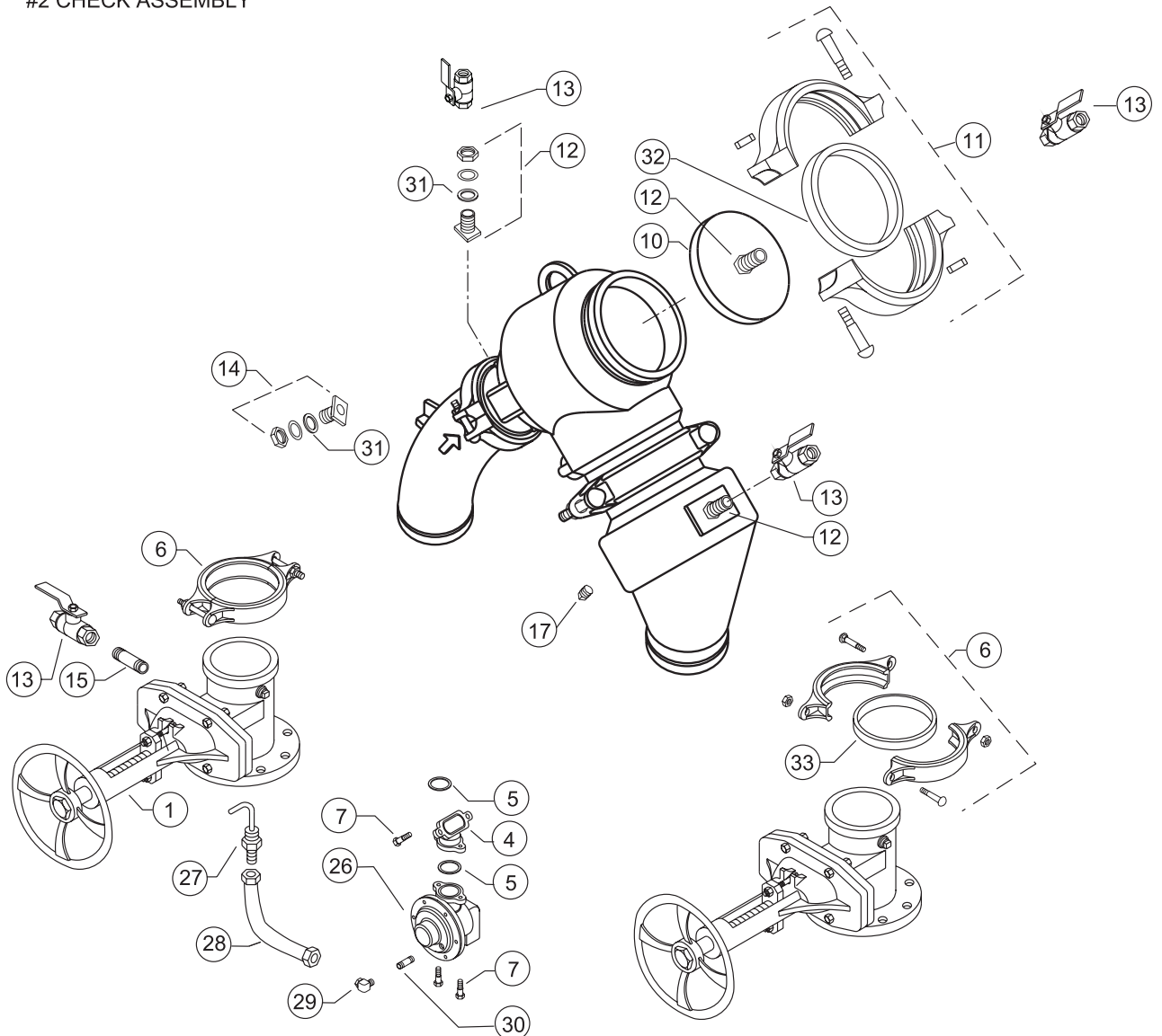
#2 CHECK ASSEMBLY
