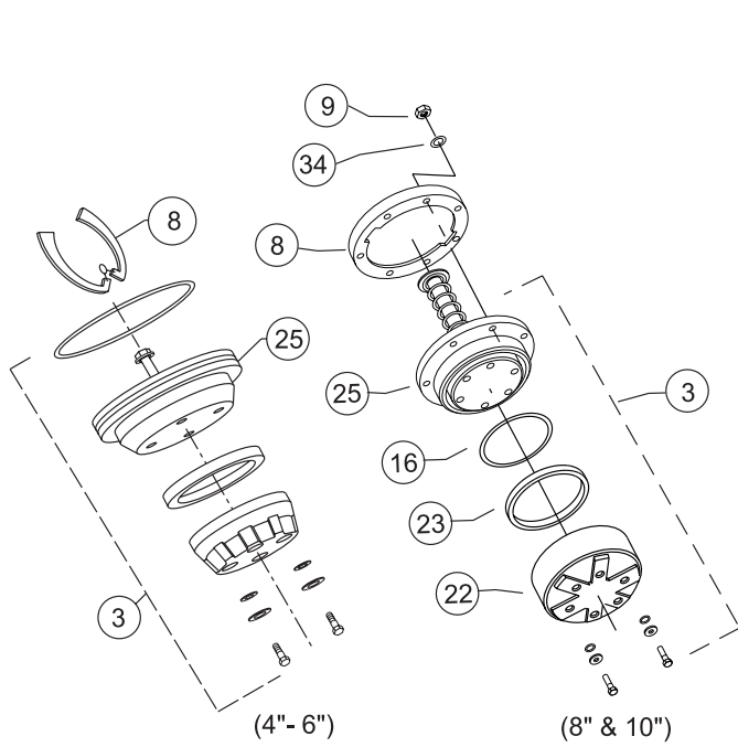
#2 CHECK ASSEMBLY
