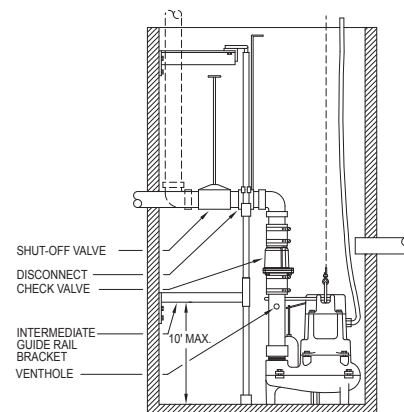
39-0003, 1½" NPT 39-0004, 2" NPT Pipe rails, pull rods and intermediate brackets not included.
