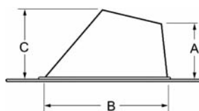
RTF Tall Cone Roof Flashing
