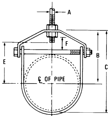
FIG. 11 STANDARD CLEVIS HANGER, DOMESTIC FIG. 11GI STANDARD CLEVIS HANGER, ELECTRO-GALVANIZED
