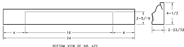
BOTTOM VIEW OF NO. 472
