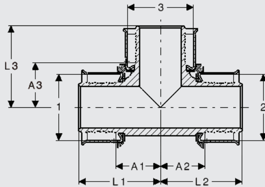
PEX Press Tees / Reducing Tees
