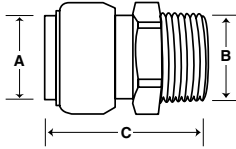
Connector Dimensions
