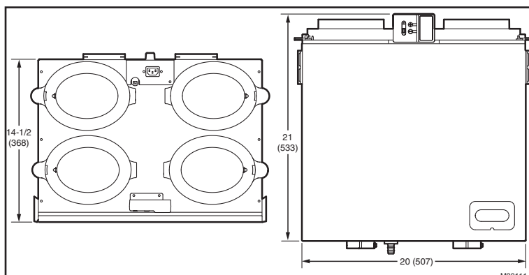
Fig. 1. Dimensions in in. (mm) and clearances.
