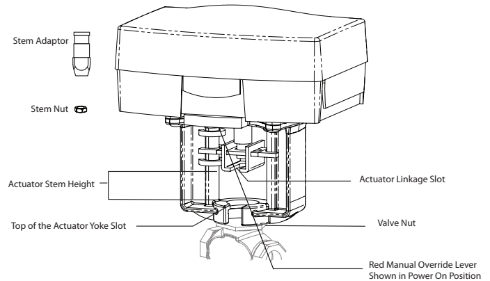
Screw-Mount Forta
