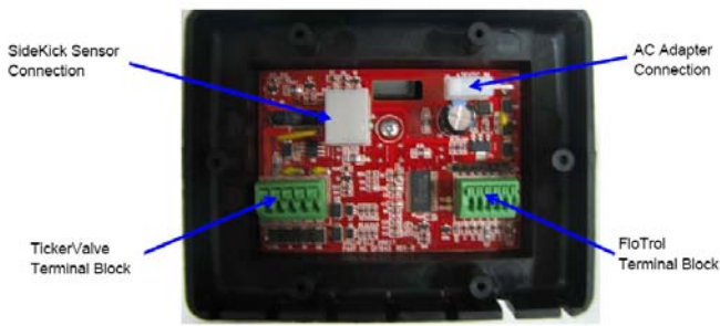
VIP Jr. Circuit Board
