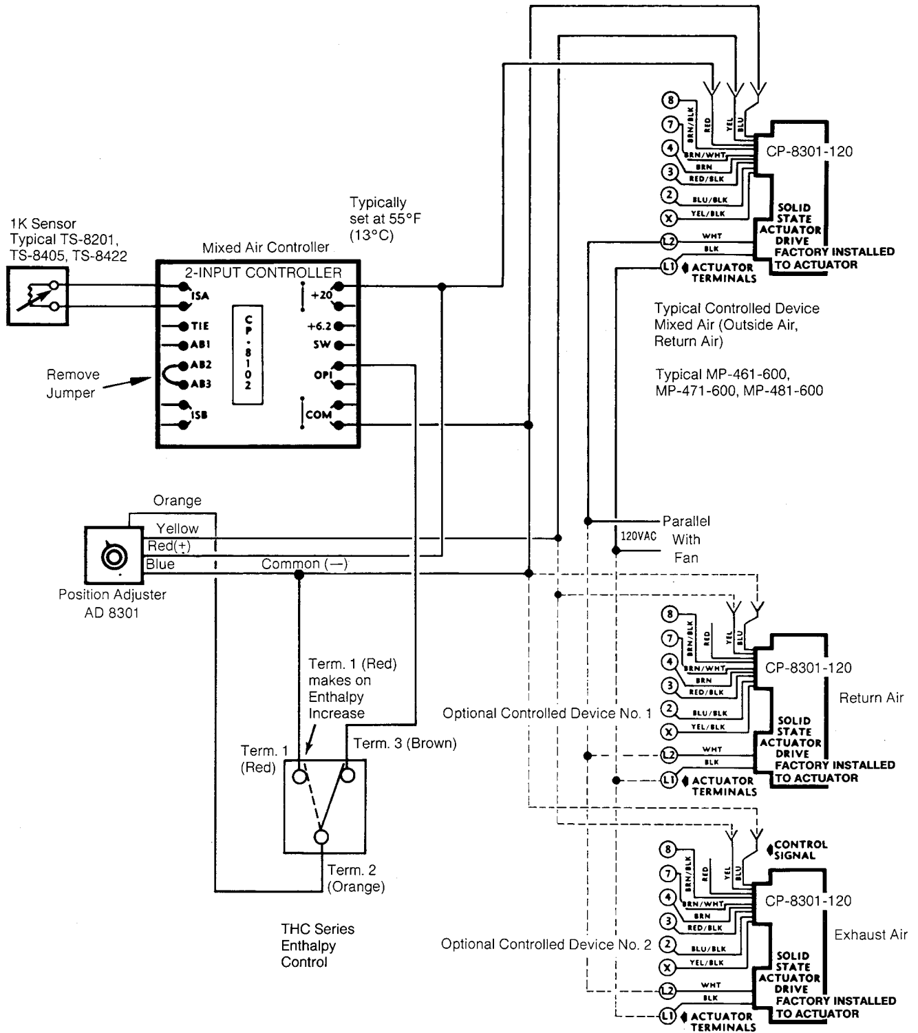
Figure-12 Economizer Cycle Using TAC System 8000 and Enthalpy Controls.
