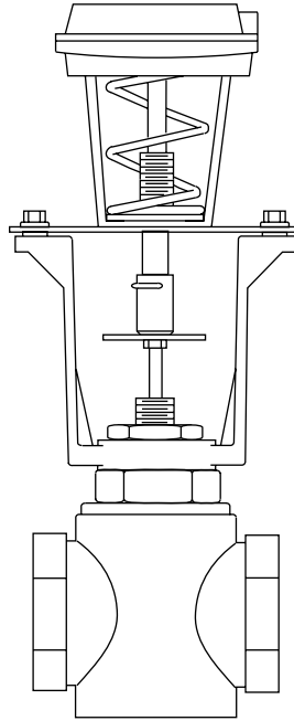
Figure-4 Typical MK-47X1 Series Actuator Using the AV-430 Valve Linkage.
