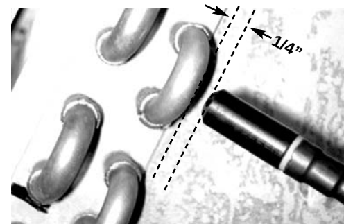
SRL8 testing an A-coil in an evaporator, 1/4" from the line.
