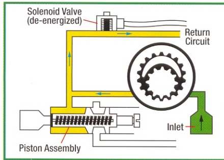
CleanCut Pump — start-up
