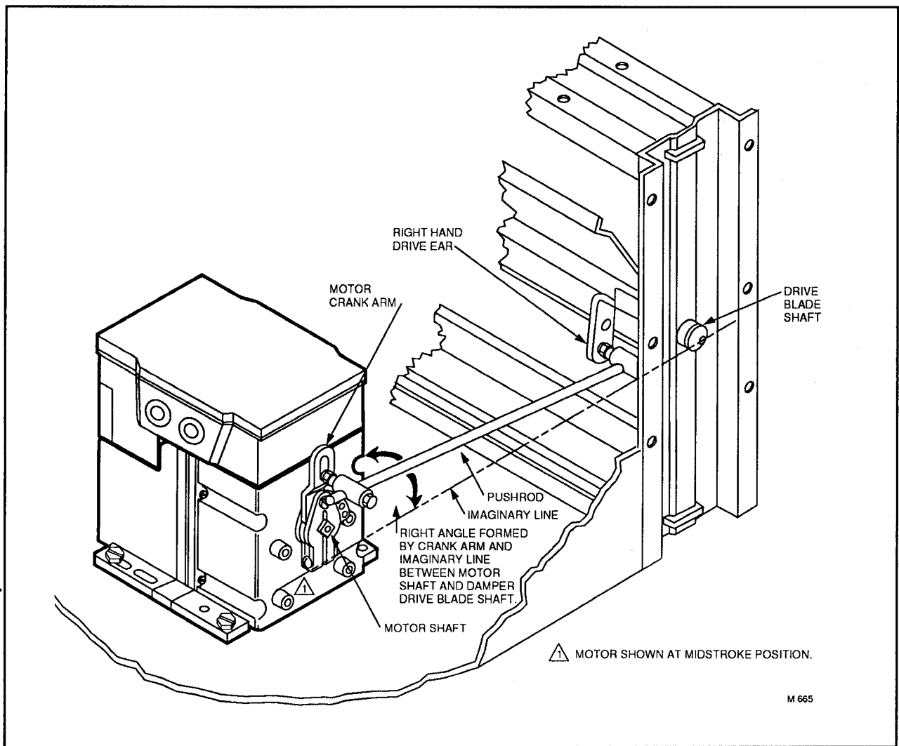
FIG. 10—ORIENTATE MOTOR CRANK ARM TO THE PROPER MIDSTROKE POSITION.
