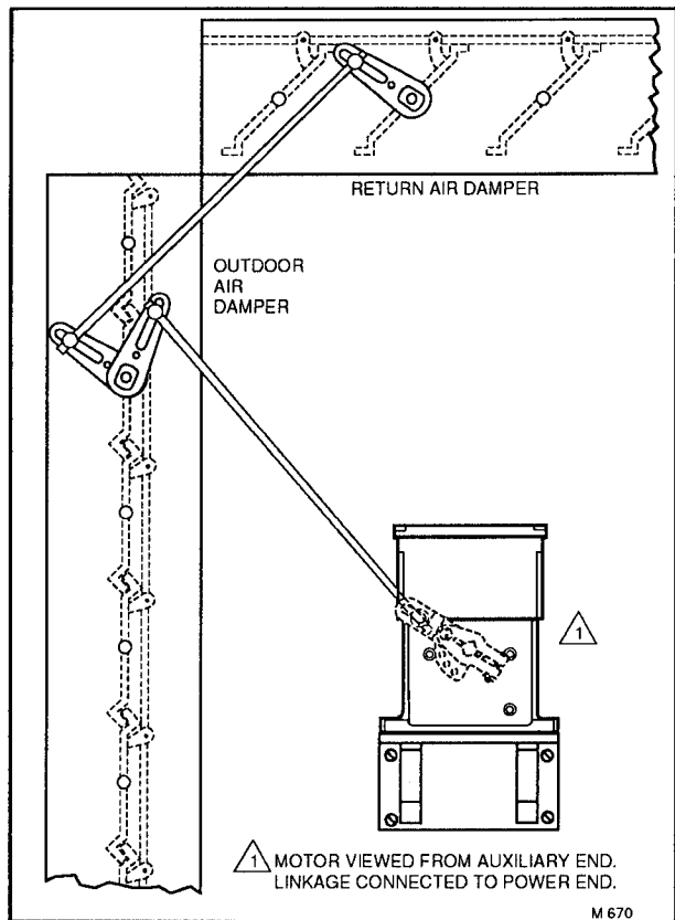
FIG. 16—MODUTROL MOTOR MOUNTED EXTERNALLY ON THE DUCT TO CONTROL TWO DAMPERS ACTING AT RIGHT ANGLES.
