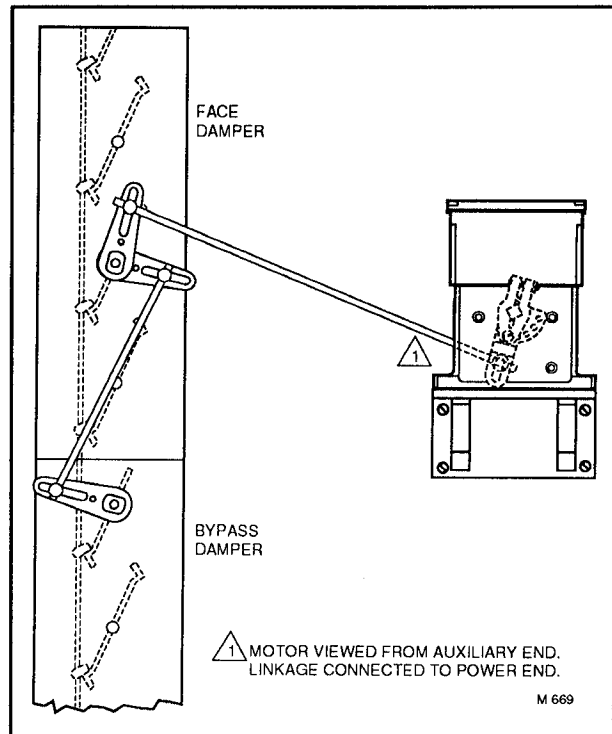
FIG. 15—MODUTROL MOTOR MOUNTED EXTERNALLY TO OPERATE A NORMALLY CLOSED FACE DAMPER AND A NORMALLY OPEN BYPASS DAMPER.
