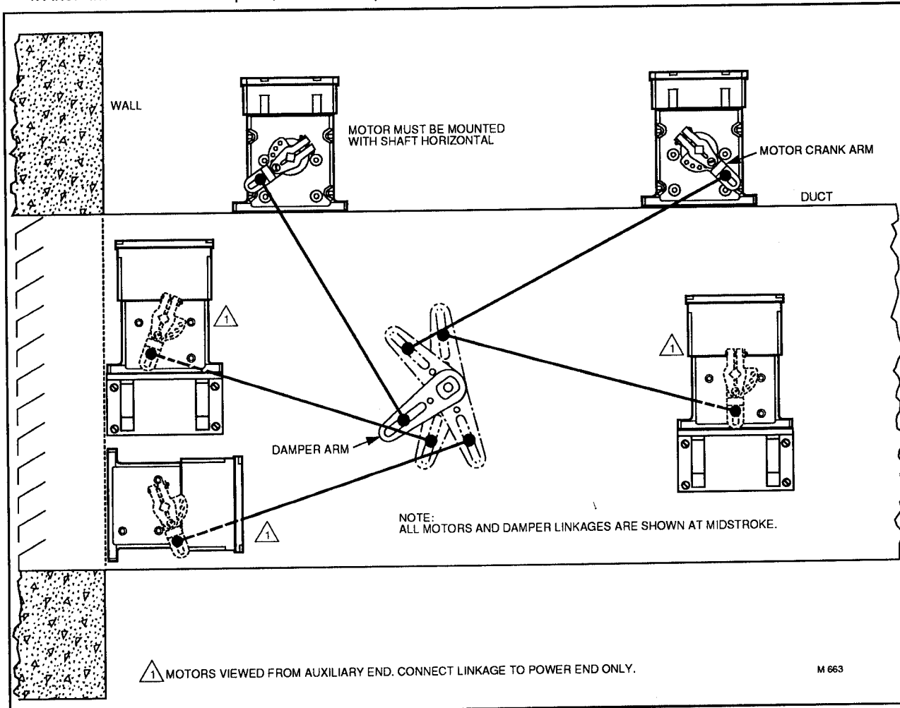
FIG. 5—MODUTROL MOTOR MUST BE MOUNTED WITH SHAFT HORIZONTAL.
