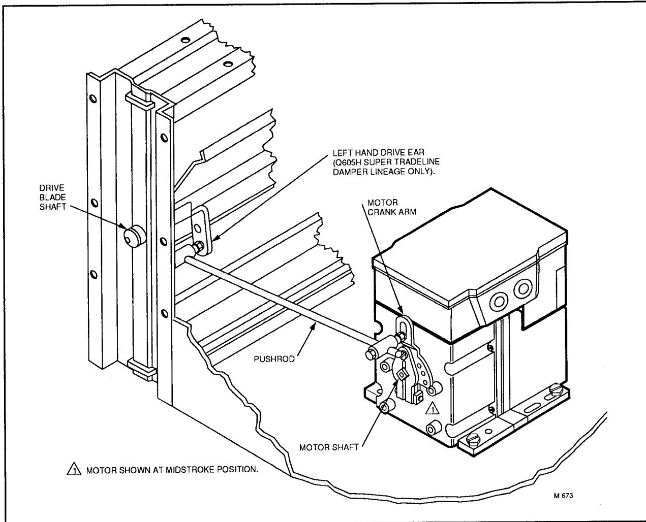
FIG. 19—MODULATING OPERATION OF A NORMALLY OPEN DAMPER, POSITION ADAPTER ARM SAME AS CRANK ARM ABOVE.
