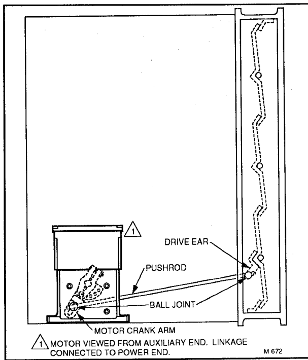
FIG. 18—TWO-POSITION OPERATION (WITHOUT ADAPTER ARM) OF A NORMALLY OPEN DAMPER.
