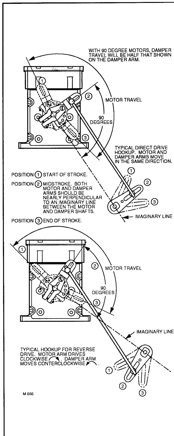
FIG. 12—POSITIONING THE LINKAGE. NOTE THAT MOTOR ARM POSITIONS SHOWN ARE TYPICAL; THE EXACT POSITION OF THE MOTOR ARM MAY BE ANYWHERE ON THE SHAFT, DEPENDING ON DAMPER LOCATION.
