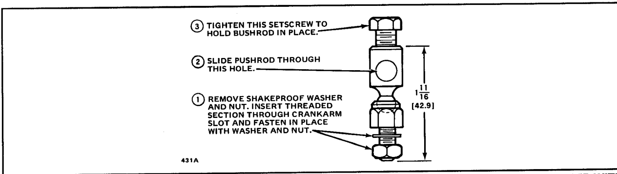
FIG. 4—DIMENSIONS IN ins. [mm IN BRACKETS] AND INSTALLATION OF 27518 BALL JOINTS FURNISHED WITH ALL LINKAGES.
