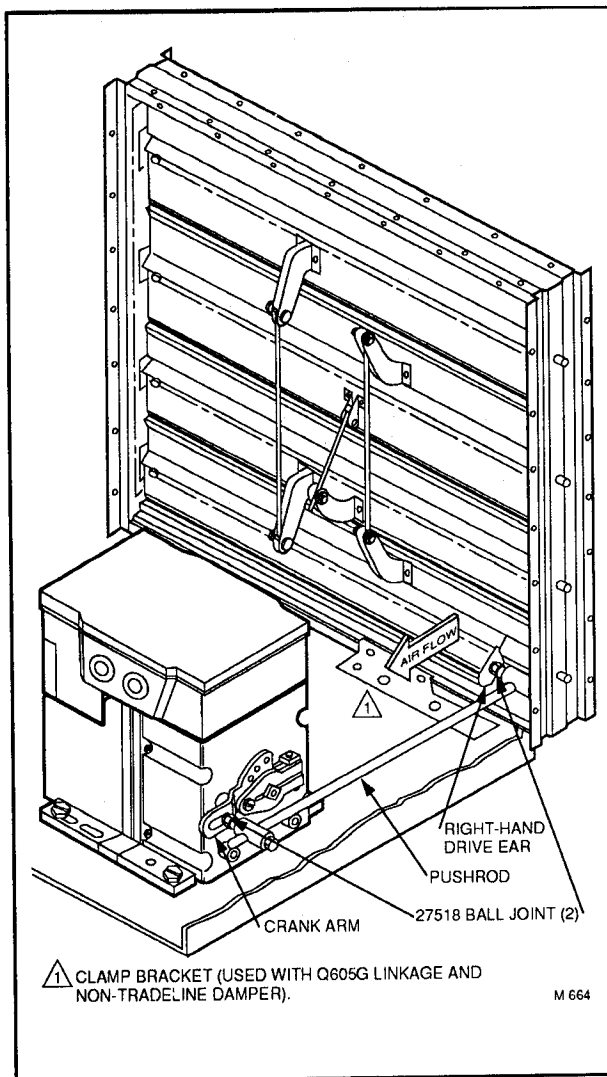
FIG. 8—MOUNTING MOTOR INTERNALLY WITH A HORIZONTAL DAMPER.
