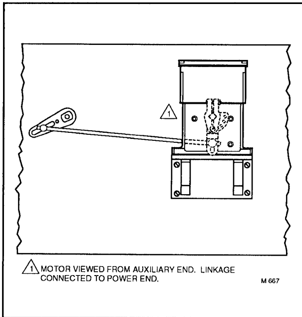
FIG. 13—MODUTROL MOTOR MOUNTED EXTERNALLY ON THE DUCT TO CONTROL ONE DAMPER.
