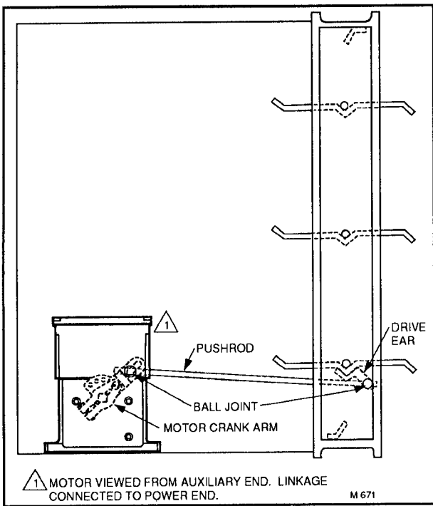
FIG. 17—TWO-POSITION OPERATION (WITHOUT ADAPTER ARM) OF A NORMALLY CLOSED DAMPER.
