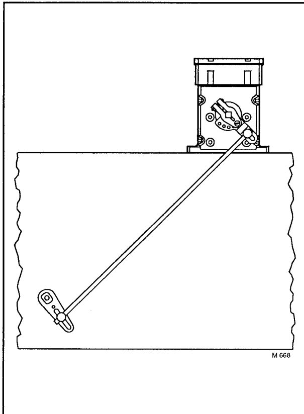
FIG. 14—MODUTROL MOTOR MOUNTED DIRECTLY ON THE DUCT (WITHOUT A MOUNTING BRACKET) TO CONTROL ONE DAMPER.
