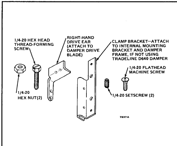
FIG. 6—PARTS INCLUDED IN 191385 INTERNAL MOUNTING KIT. INTERNAL MOUNTING.
