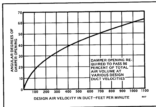
FIG. 9—USE THIS CURVE WHEN DETERMINING INITIAL DAMPER SETTINGS.
