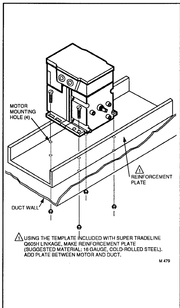
FIG. 7—IF MOUNTING A MOTOR INSIDE A THIN WALLED DUCT, ADD A REINFORCEMENT PLATE.
