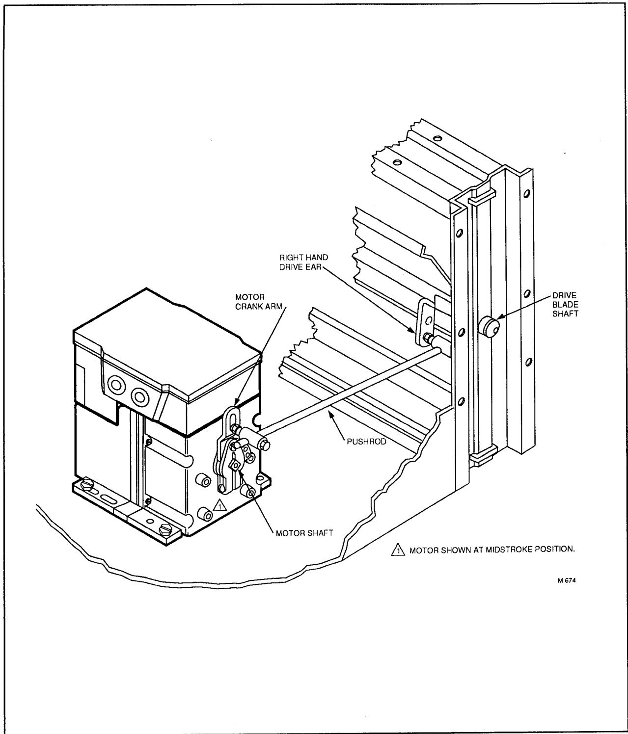
FIG. 20—MODULATING OPERATION OF A NORMALLY CLOSED DAMPER. POSITION ADAPTER ARM SAME AS CRANK ARM ABOVE.
