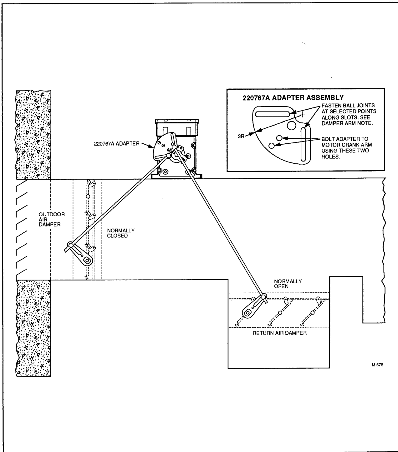
FIG. 21—MOTOR MOUNTED EXTERNALLY ON THE DUCT TO CONTROL TWO DAMPERS ACTING AT RIGHT ANGLES. USE OF ADAPTER ASSEMBLY ELIMINATES ONE DAMPER ARM, AND ALSO MAKES POSSIBLE THE USE OF TWO PUSH RODS OF NEAR EQUAL LENGTH INSTEAD OF ONE SHORT ROD AND THE OTHER TOO LONG TO BE PRACTICAL.
