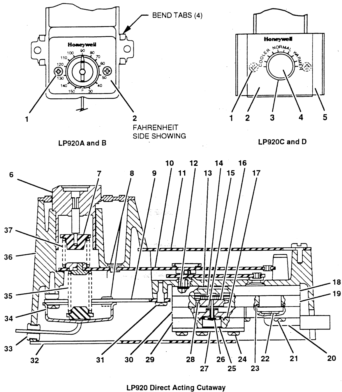
Fig. 10. (Part 1 of 2). LP920 Remote Bulb Temperature Controller.
