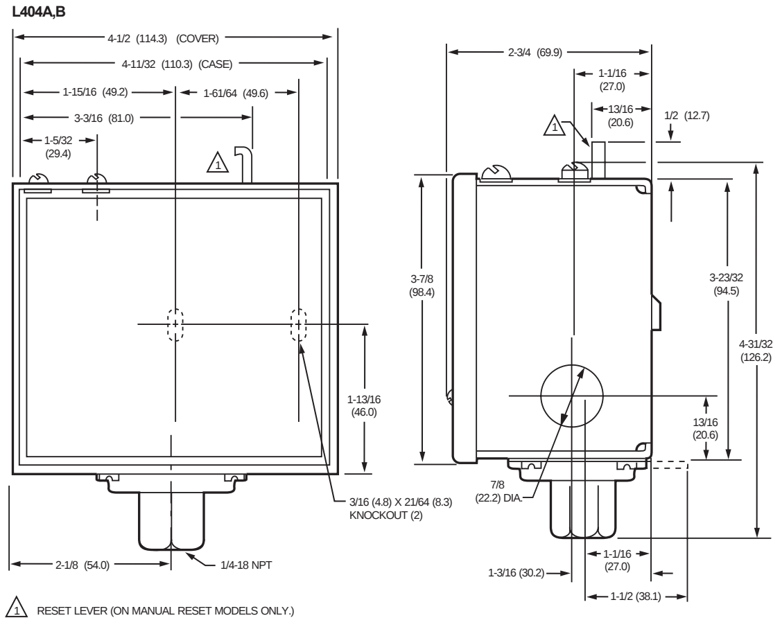
Fig. 1. Mounting dimensions of the L404A,B Pressuretrol® Controllers in in. (mm).
