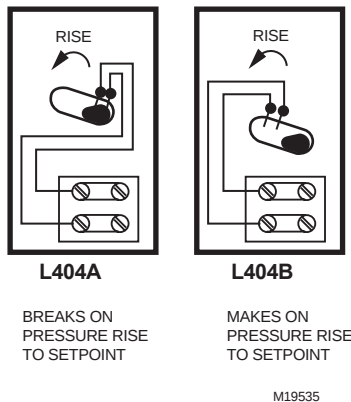
Fig. 3. L404 terminal blocks and internal schematics.
