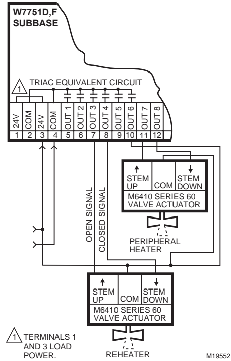
Fig. 11. M6410A Actuator wired with W7751D,F Controller.
