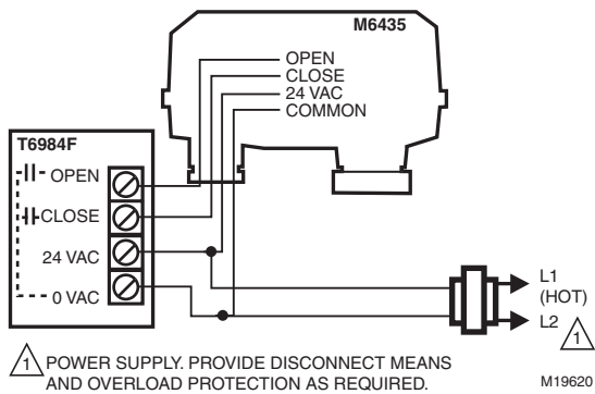
Fig. 8. M6435A used with T6984F.
