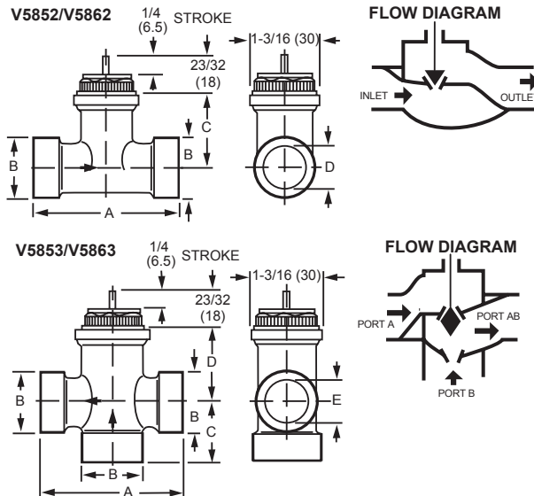
Fig. 1. Dimensions of V5852A, V5853A, V5862A and V5863A in in. (mm).
