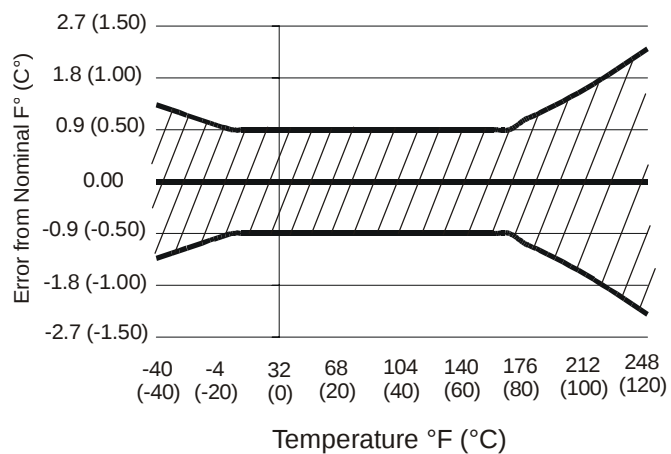
Figure 12: Sensor Accuracy
