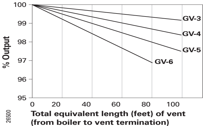
Figure 2 Boiler output
