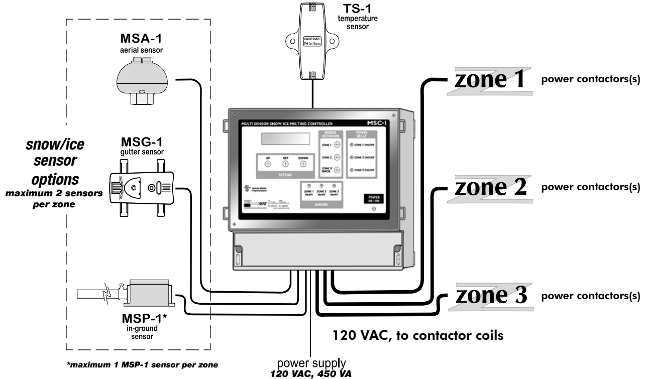
Fig.2 Sample Application Illustration
