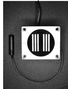
In-ground Sensor, MSP-1: installed in-ground to detect moisture and slab temperature (the MSC-1 must be programmed to recognize this sensor, refer to the instruction manual for details).
