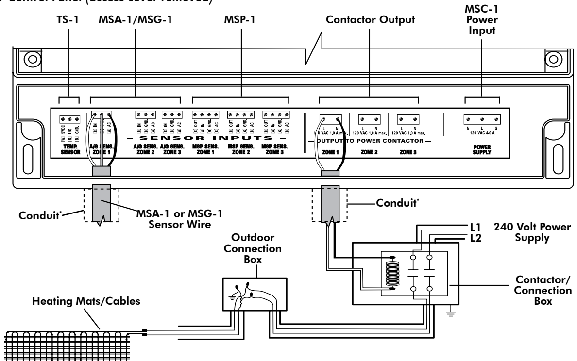
Fig.4 MSC-1 Control Panel (access cover removed)
