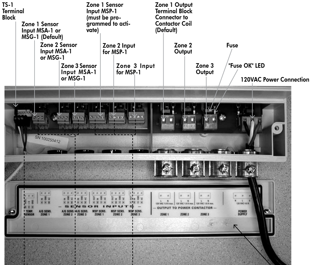
Fig.4 MSC-1 Control Panel (access cover removed)
