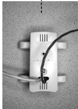
Gutter Sensor, MSG-1: secured in the gutter to detect moisture conditions (may be used as the preprogrammed sensor).
