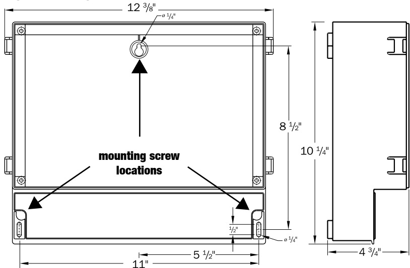
Fig.3 Mounting: mounts to wall via three #10 screws
