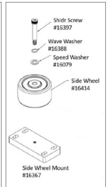
Figure C. Mounting block has slots on mounting screw holes.
