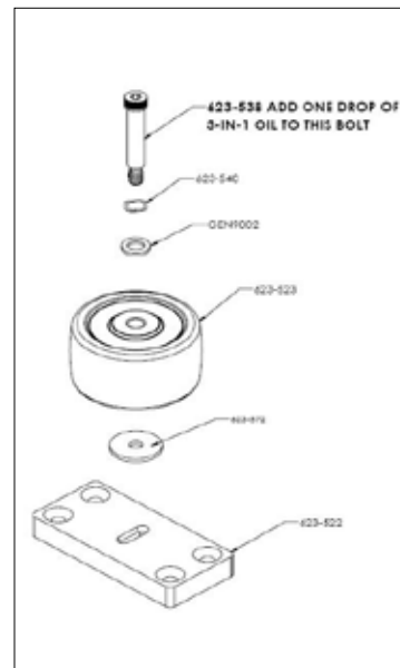
Figure B. Mounting block with slot in the center.
